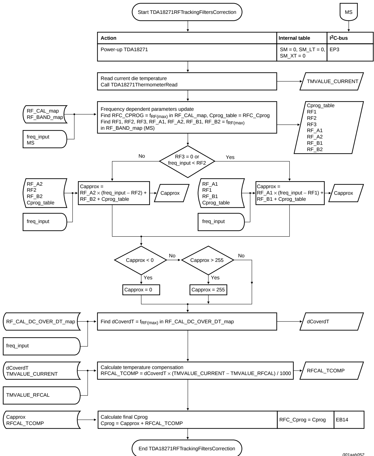
Fig 16. Flowchart TDA18271RFTrackingFiltersCorrection
